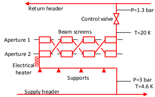
Figure 1: LHC beam screen cooling scheme
